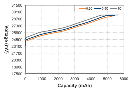
Rate charge curve@ 25°C
