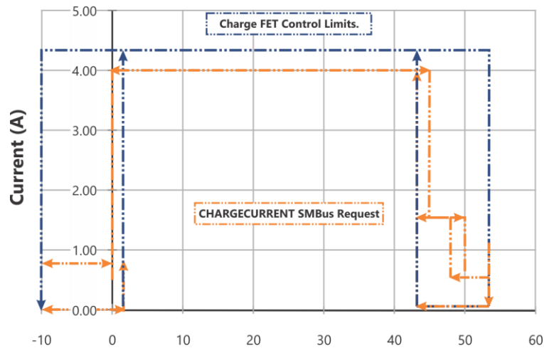
Charge Operating Limits
