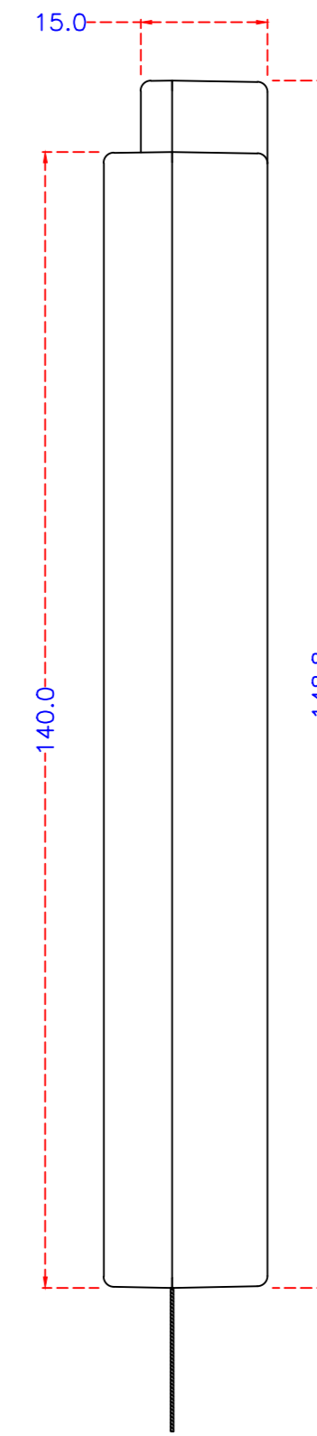
SIDE VIEW OUTLINE
