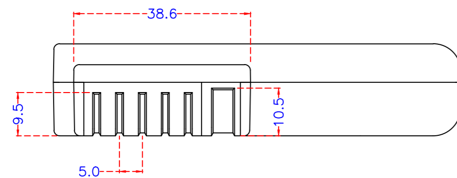
FRONT VIEW OUTLINE
