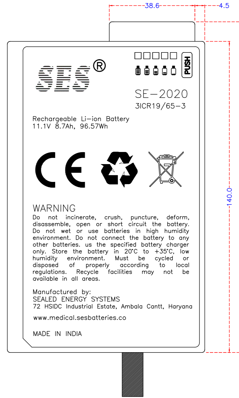
TOP VIEW OUTLINE
